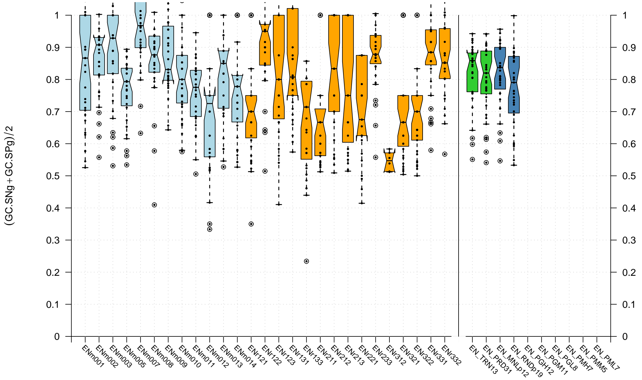
Gene (Coding Exons) Level : boxplot for (GC.SNg + GC.SPg) / 2
